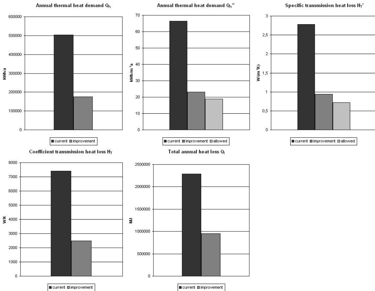
Fig. 6 Graphs showing improvements regarding heat demand and loss.
