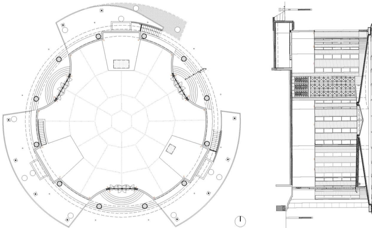
Fig. 2 The French Pavilion, ground-floor plan and section (contract design, 2010).
