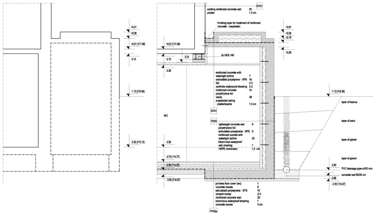
Fig. 4. Longitudinal sections through one of the basement segments showing the uninsulated perimeter walls and slabs documented by an architectural survey (2007, left) and insulation and drainage layers implemented in the contract design (2010, right).
