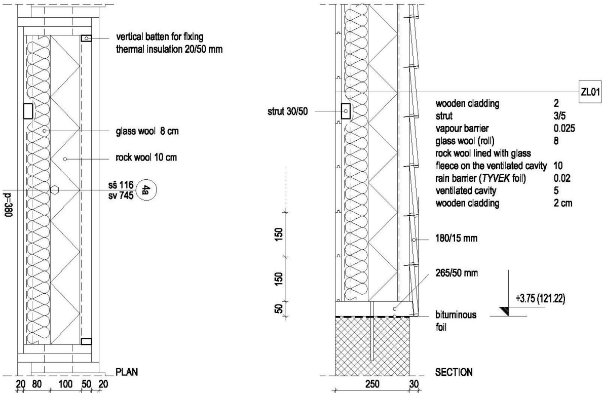
Fig. 3 The Plan and section of perimeter wooden walls showing the application of thermal insulation and supporting layers within the cavity of wooden panels.
